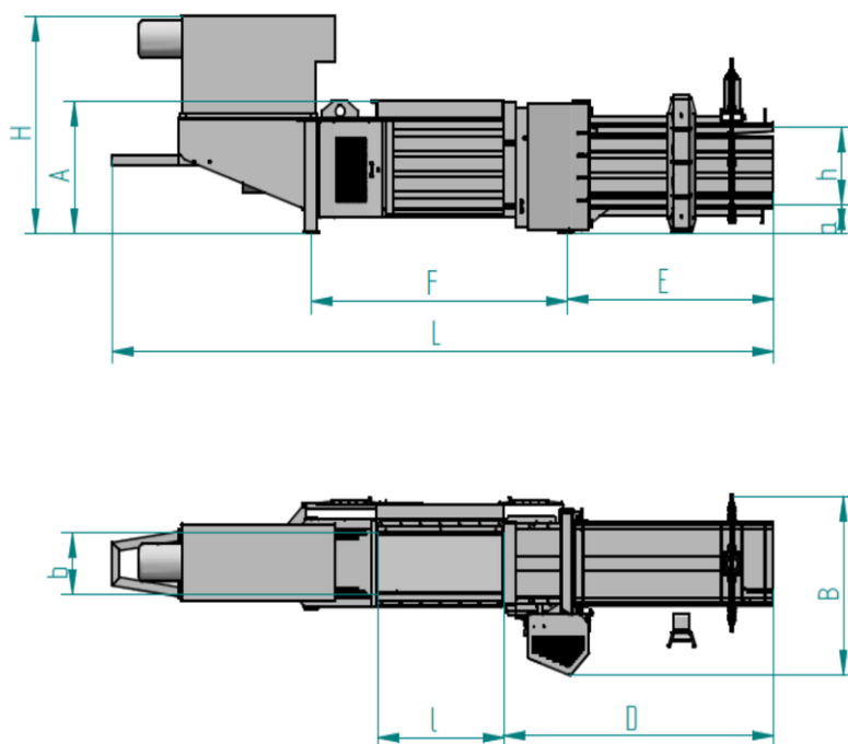
HPK 750 H
